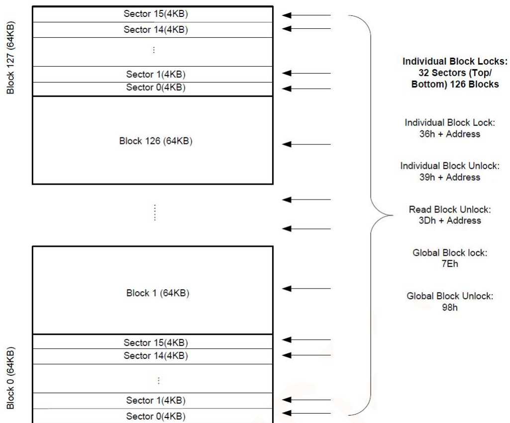
Figure 6.2 Individual Block/Sector Locks
