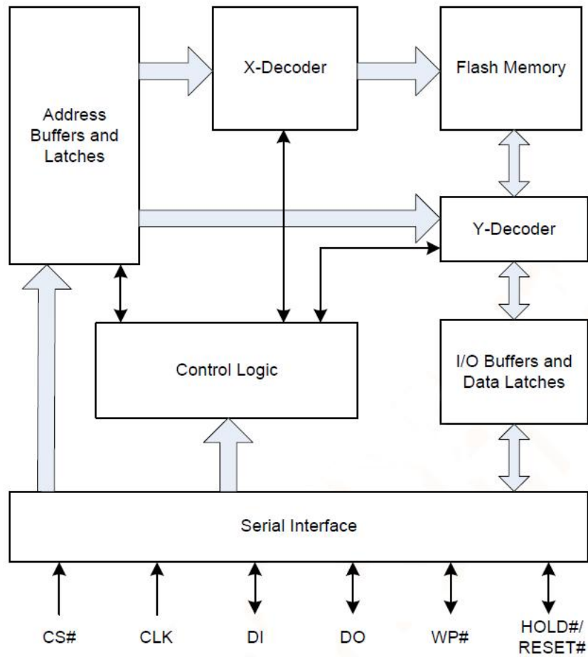
Figure 2.1 Block Diagram
