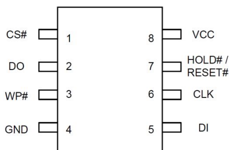
Figure 3.1 SOP8 (208mil)
