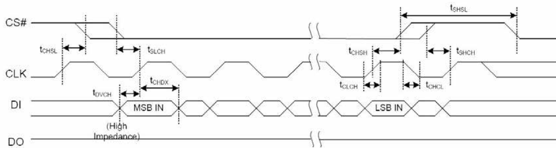
Figure 8.5 Input Timing
