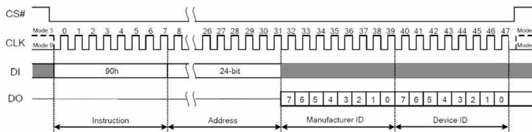
Figure 7.30a Read Manufacturer/Device ID(SPI Mode)
