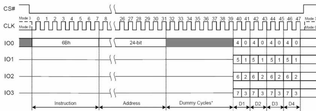
Figure 7.16 Fast Read Quad Output Instruction
