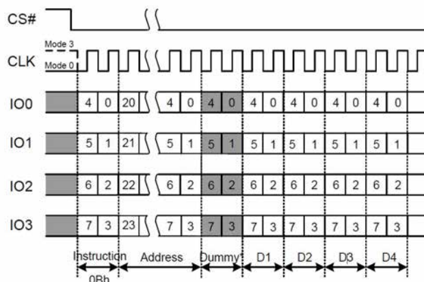
Figure 7.14b Fast Read Instruction (QPI Mode)
