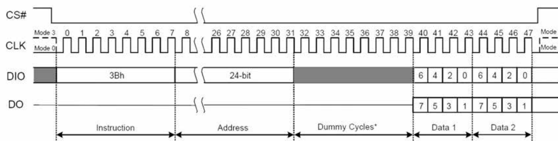
Figure 7.15 Fast Read Dual Output Instruction Sequence Diagram
