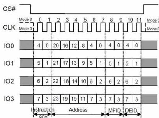
Figure 7.30b Read Manufacturer/Device ID(QPI Mode)
