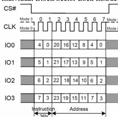
Figure 7.36b Individual Block/Sector Lock Instruction(QPI Mode)
