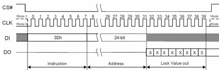
Figure 7.38a Read Block Lock Instruction(SPI Mode)
