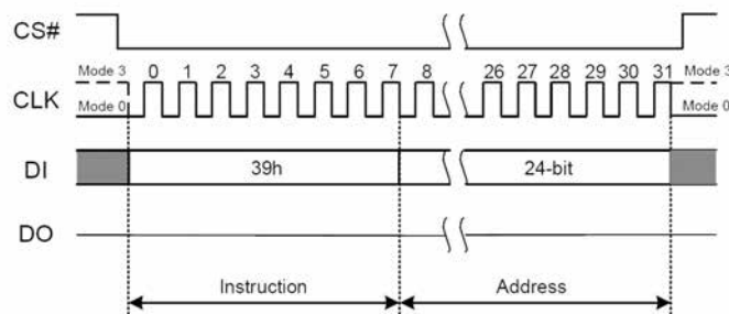
Figure 7.37a Individual Block/Sector Unlock Instruction(SPI Mode)
