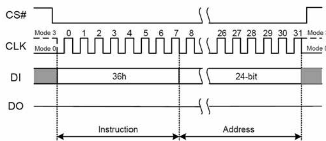
Figure 7.36a Individual Block/Sector Lock Instruction(SPI Mode)
