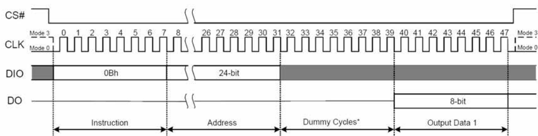
Figure 7.14a Fast Read Instruction (SPI Mode)
