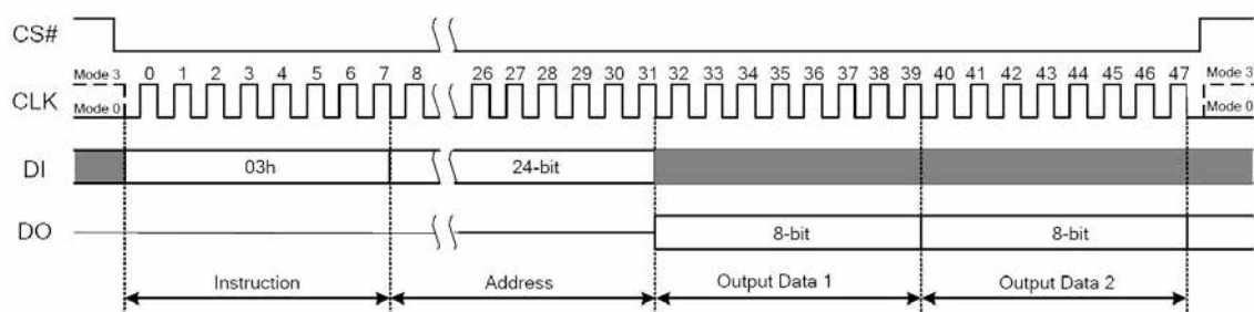
Figure 7.13 Read Data Instruction
