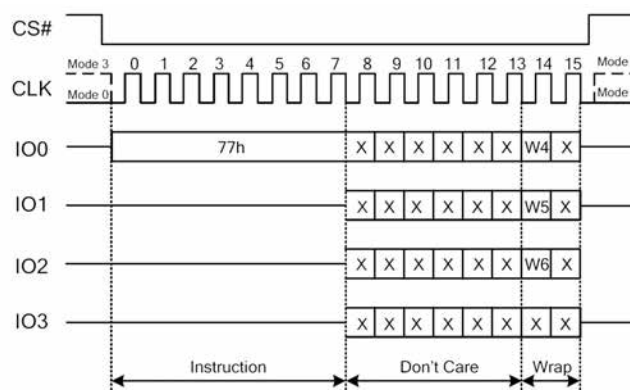
Figure 7.25 Set Burst with Wrap Instruction
