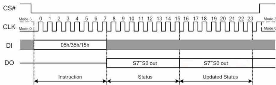
Figure 7.1a Read Status Register Instruction(SPI Mode)
