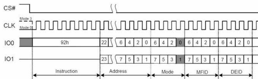
Figure 7.41 Read Manufacturer/Device ID Dual I/O Instruction
