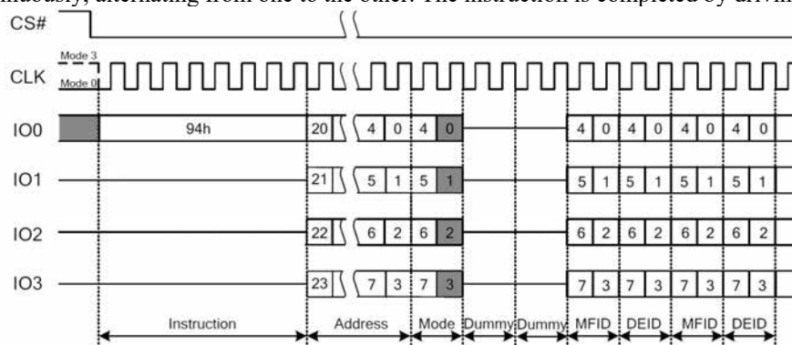
Figure 7.42 Read Manufacturer/Device ID Quad I/O Instruction
