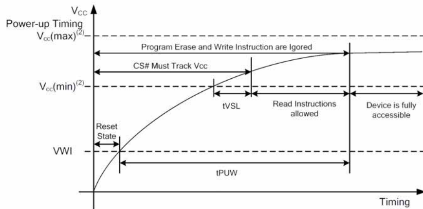
Figure 8.1 Power-up Timing
