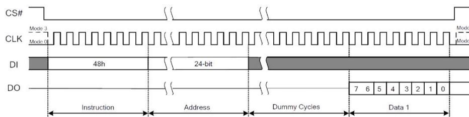
Figure 7.35 Read Security Registers Instruction
