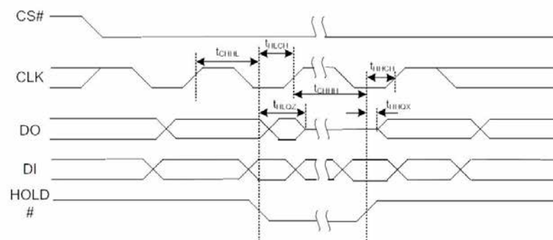
Figure 8.6 Hold Timing
