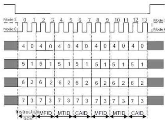
Figure 7.31b Read JEDEC ID(QPI Mode)
