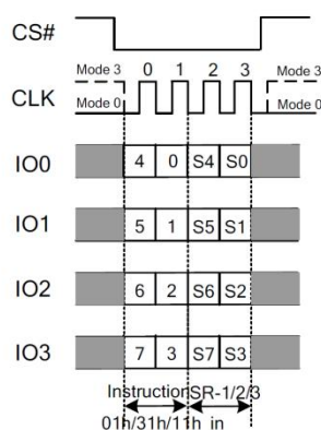
Figure 7.5b Write Status Register Instruction(QPI Mode)
