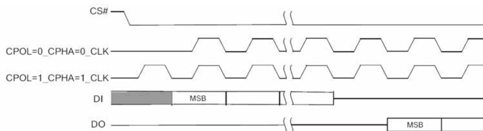
Figure 6.1 SPI Modes
