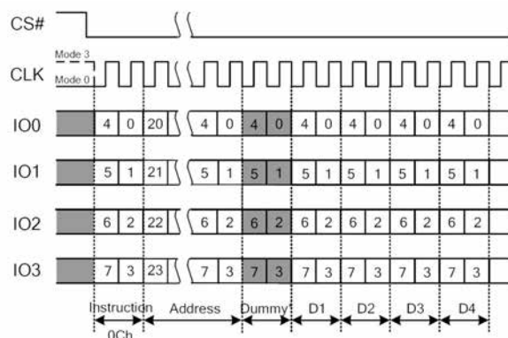
Figure 7.45 Burst Read with Wrap Instruction (QPI Mode only)
