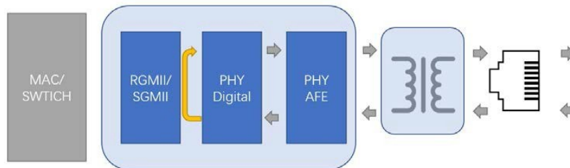
Figure 10. Remote PHY Loopback
