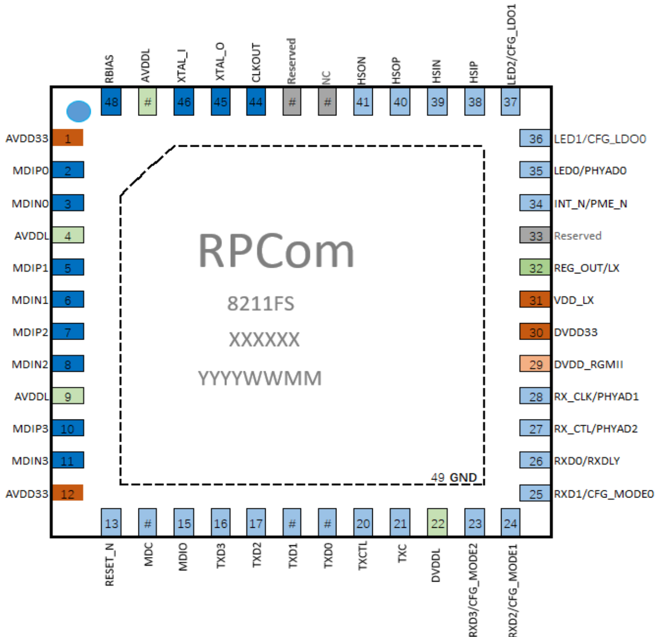
Figure 2. Pin Assignment
