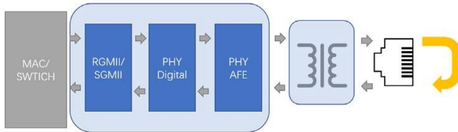
Figure 9. External Loopback
