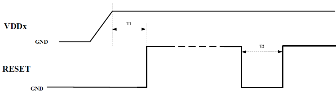
Figure 11. Reset Timing Diagram
