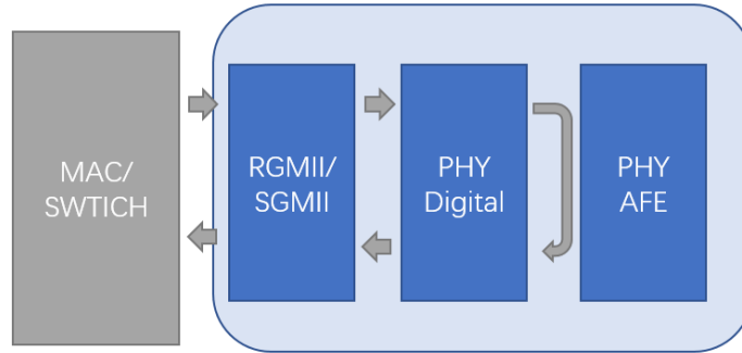
Figure 8. Digital Loopback
