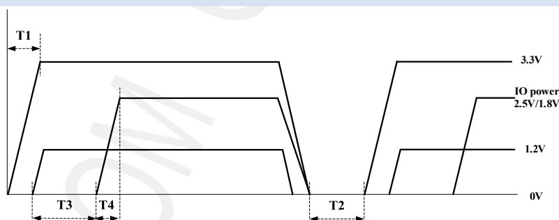
Figure 13. Power Sequence Diagram
