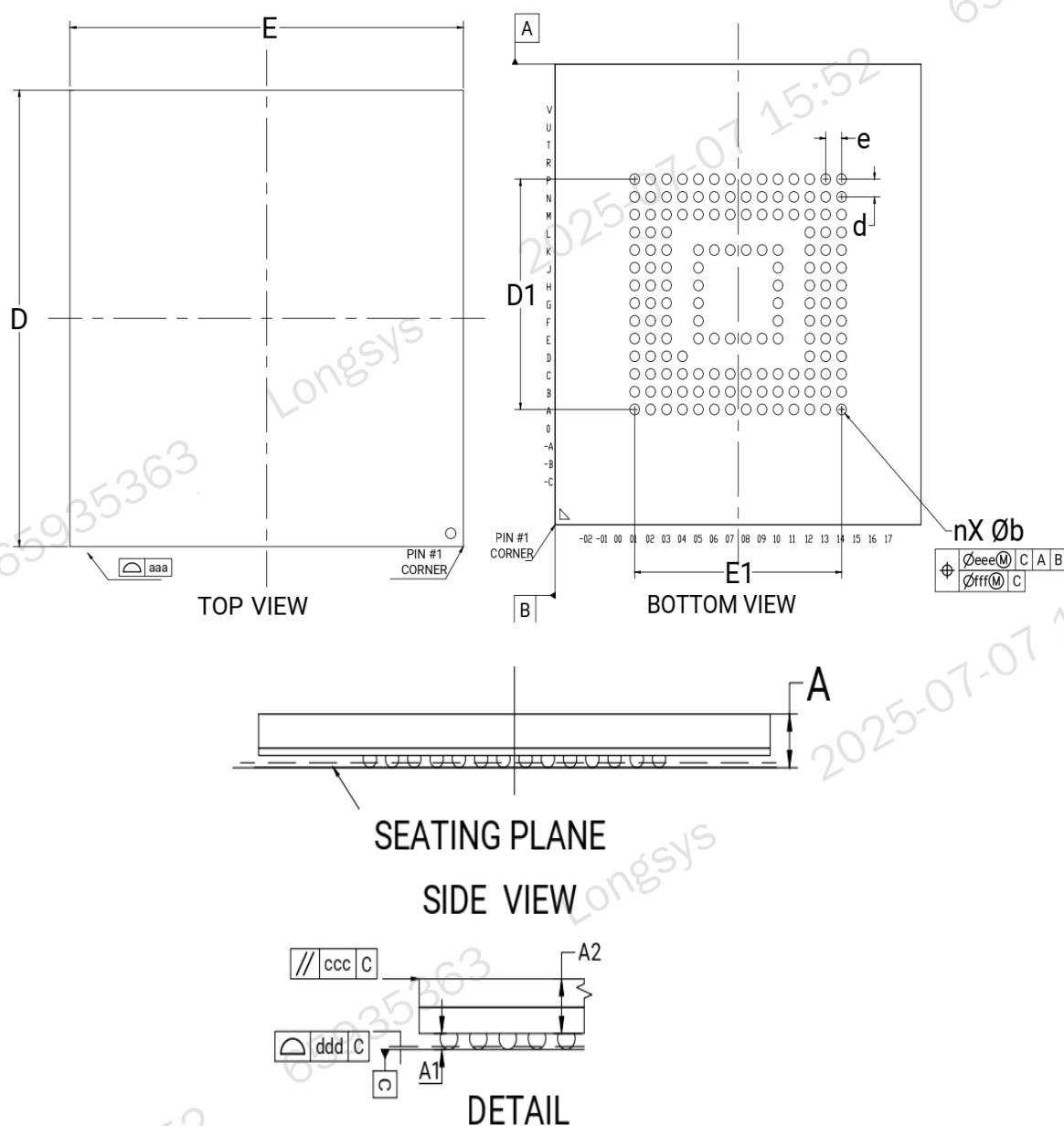
Figure 3 Package Dimension
