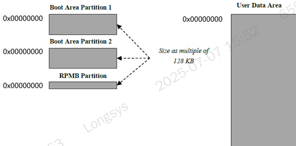
Figure 5 Partitions and User Data Area Configuration
