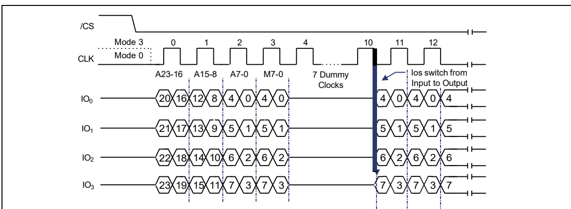
Figure 9-38 DTR Fast Read Quad I/O (Previous instruction set M5-4=10, SPI Mode)
