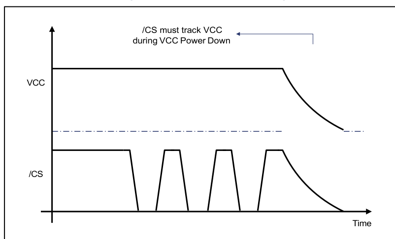
Figure 10-3 Power-Down Timing
