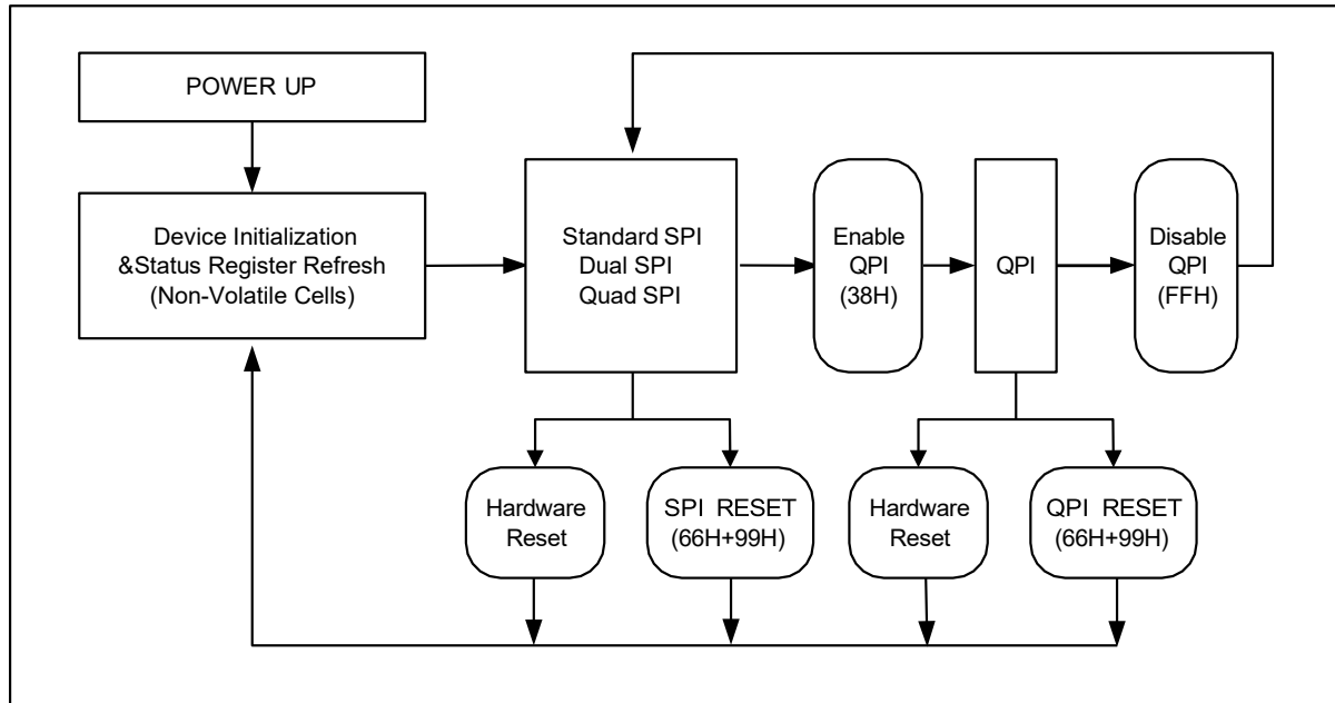
Figure 7-1 MH7256 Serial Flash Memory Operation Diagram
