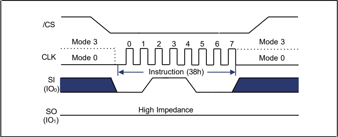
Figure 9-83 Enter QPI Instruction (SPI Mode only)
