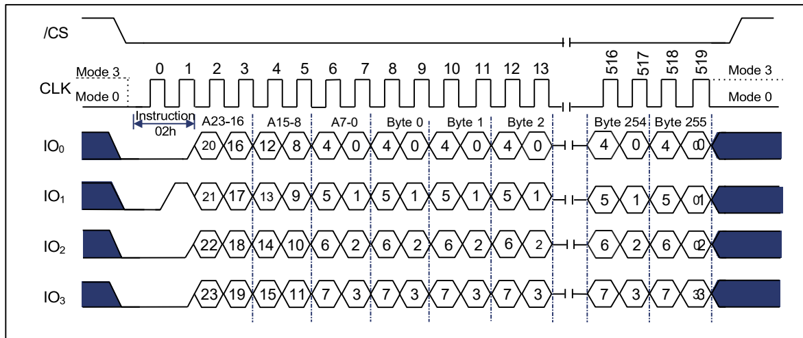
Figure 9-45 Page Program Instruction (QPI Mode)
