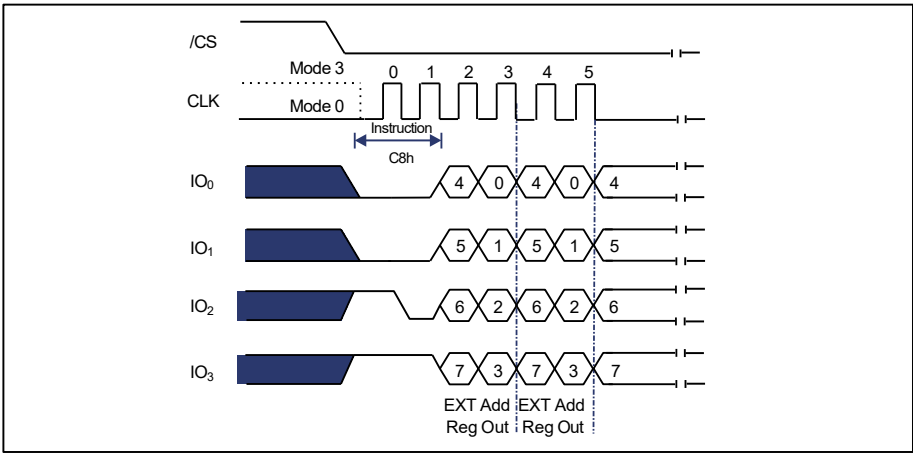
Figure 9-11 Read Extended Address Register Instruction (QPI Mode)
