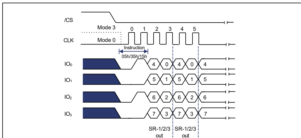
Figure 9-5 Read Status Register Instruction (QPI Mode)
