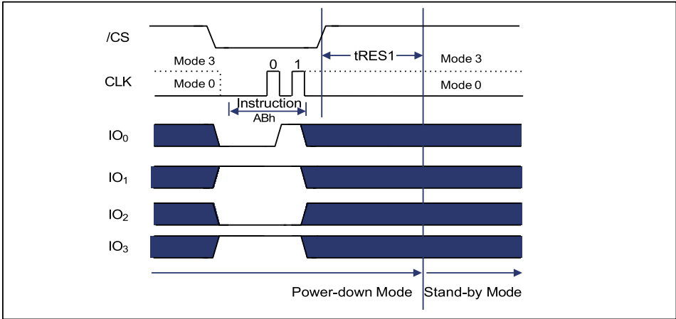
Figure 9-67 Release Power-down Instruction (QPI Mode)
