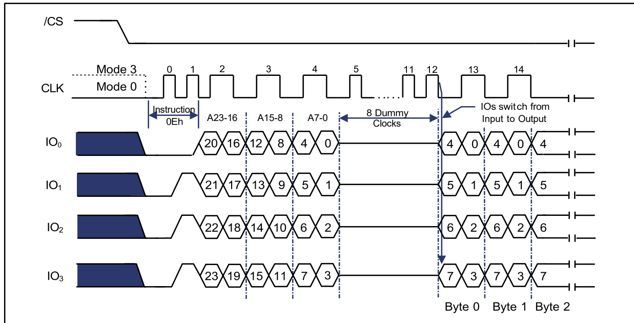
Figure 9-82 DTR Burst Read with Wrap Instruction (QPI Mode only)
