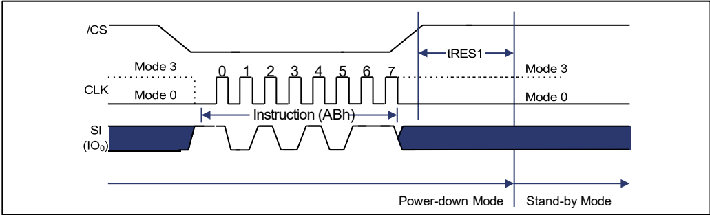
Figure 9-66 Release Power-down Instruction (SPI Mode)
