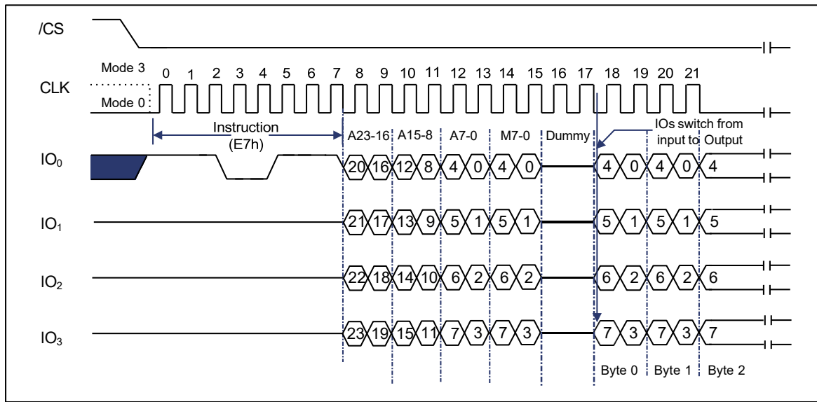
Figure 9-41 Word Read Quad I/O Instruction (Initial instruction or previous M5-4 \neq 10, SPI Mode only) 32-Bit Address is required when the device is operating in 4-Byte Address Mode
