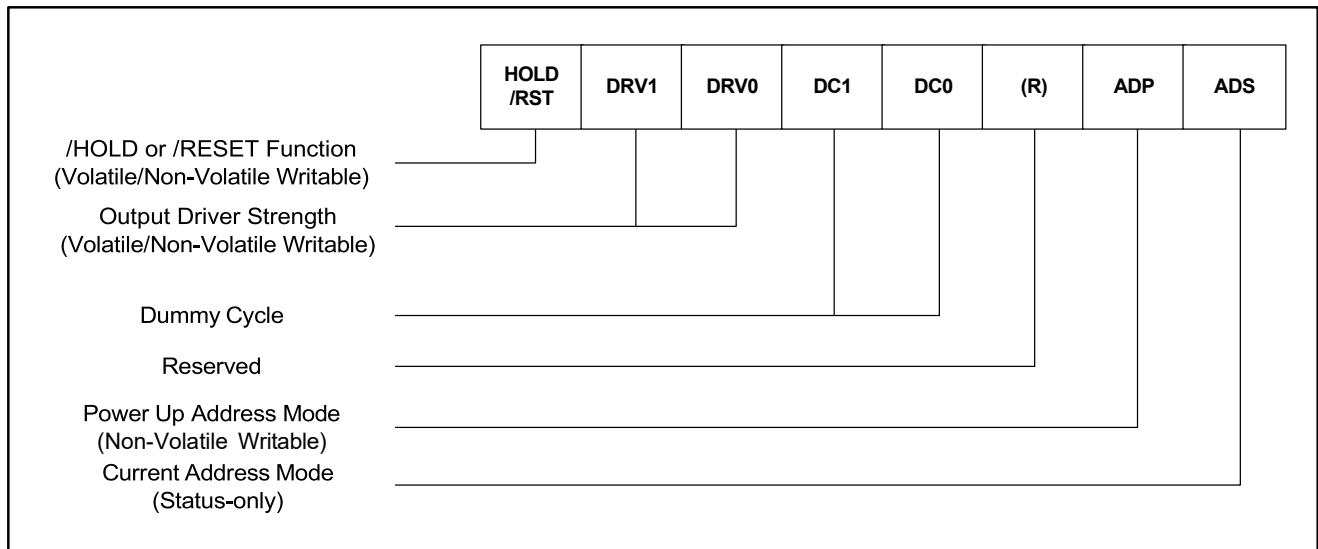
Figure 8-3 Status Register-3
