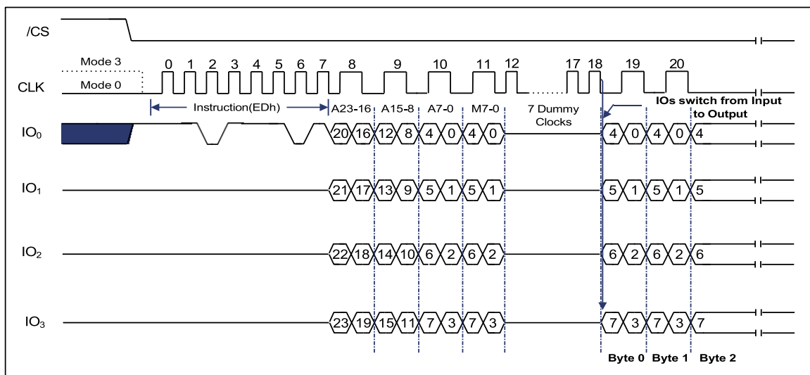
Figure 9-38 DTR Fast Read Quad I/O (Previous instruction set M5-4=10, SPI Mode)
