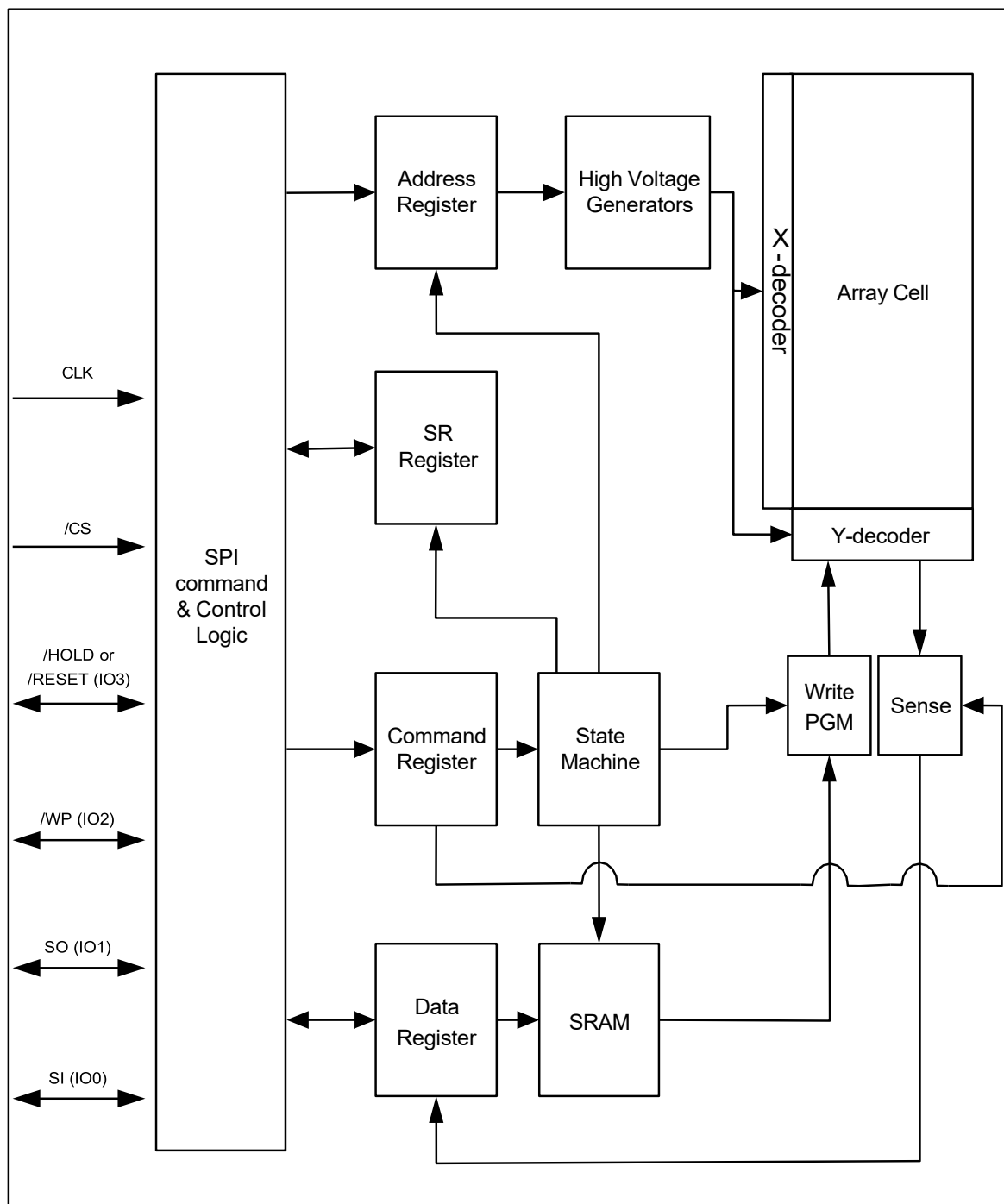
Figure 4-1 MH7256 Serial Flash Memory Block Diagram
