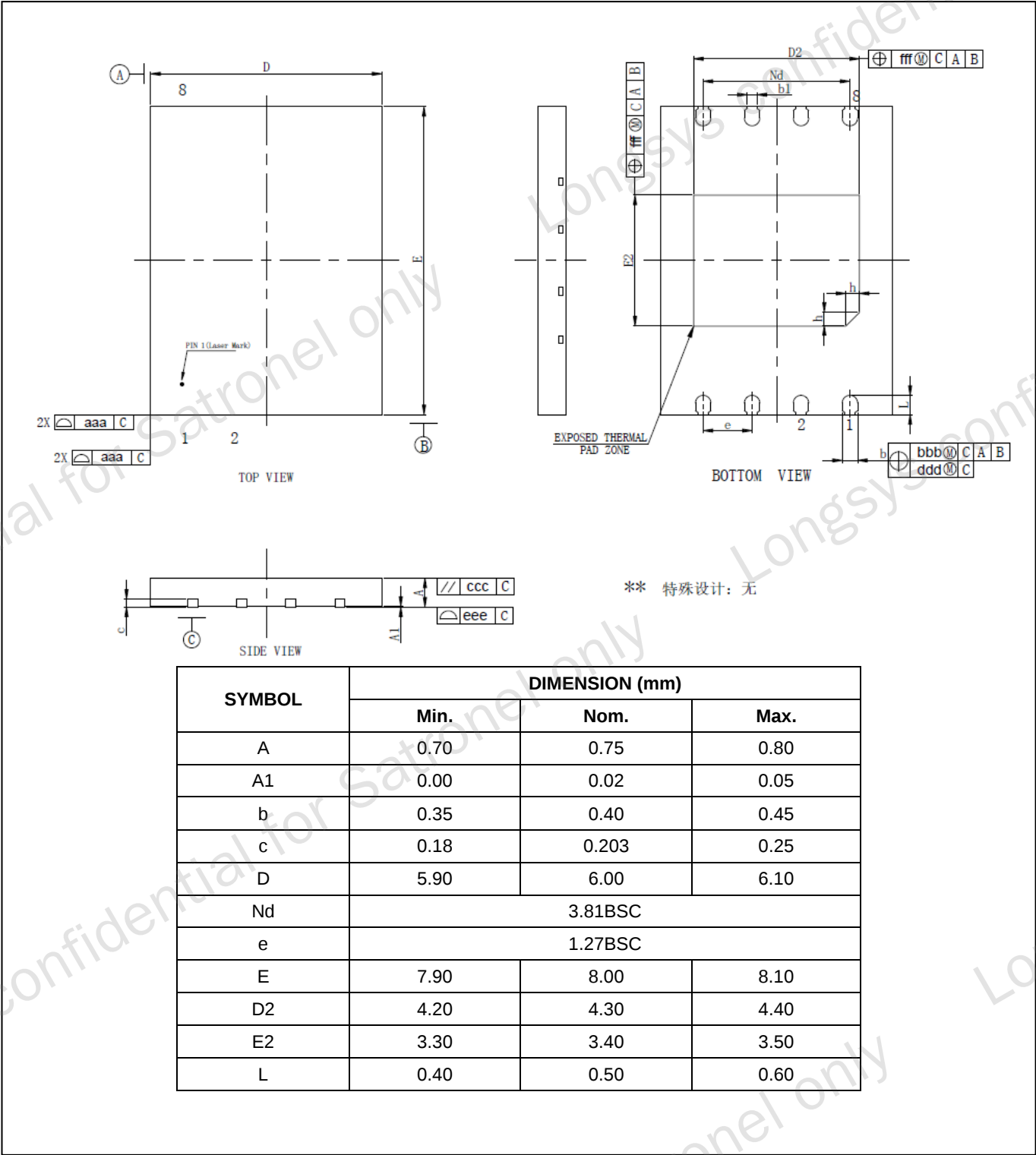
Figure 37 8-WSON (8x6mm) Package Information
