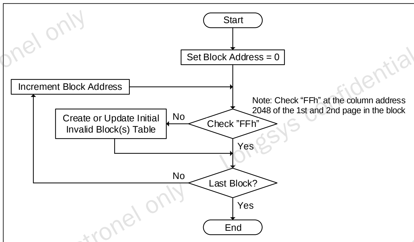
Figure 26 Flow to Create Initial Invalid Block Table
