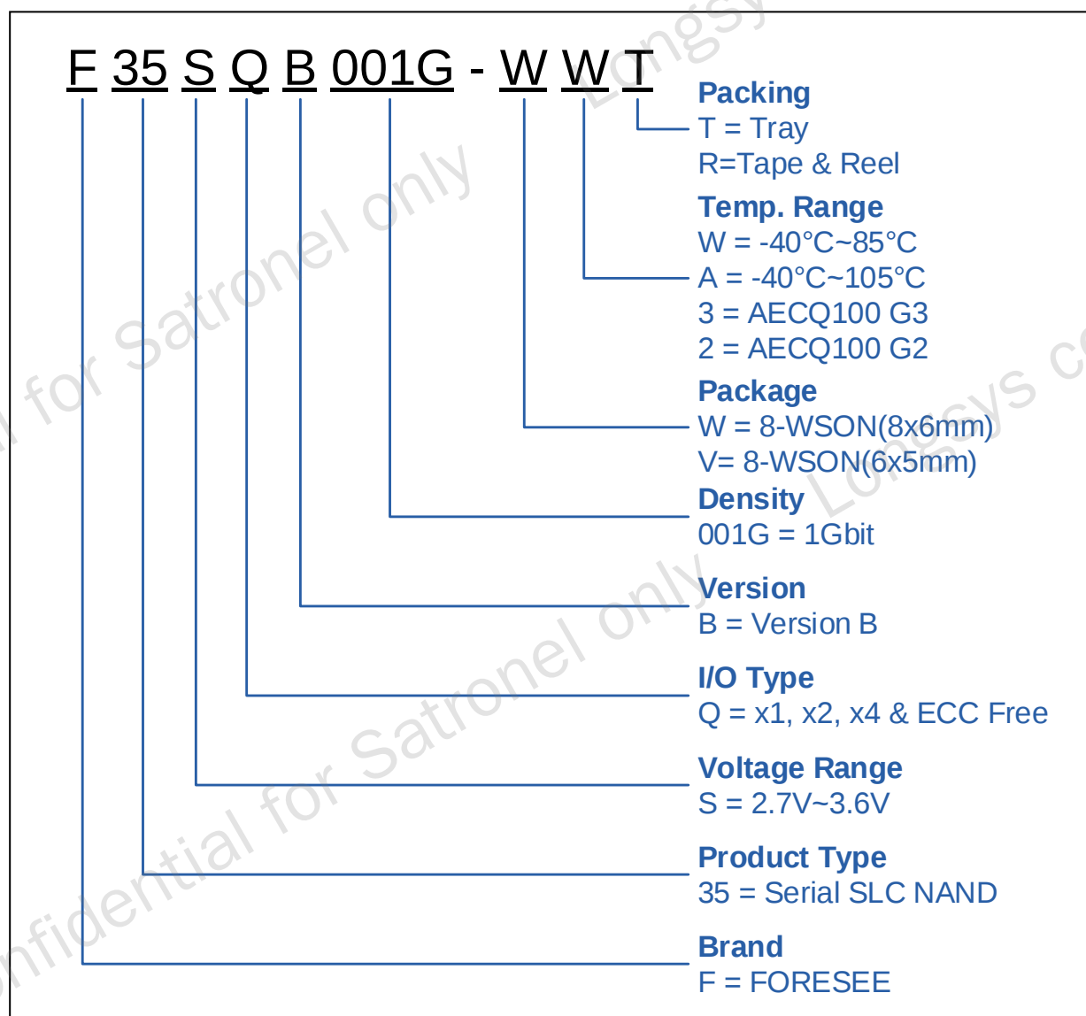
Figure 1 Marketing Part Numbering Chart
