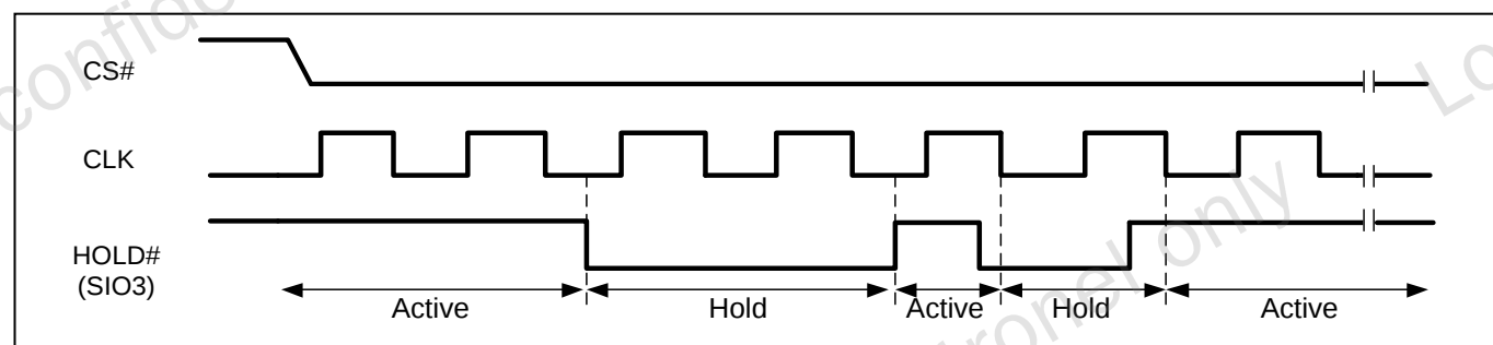
Figure 7 Hold Condition
