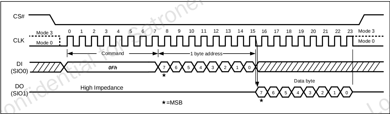
Figure 10 Get Feature
