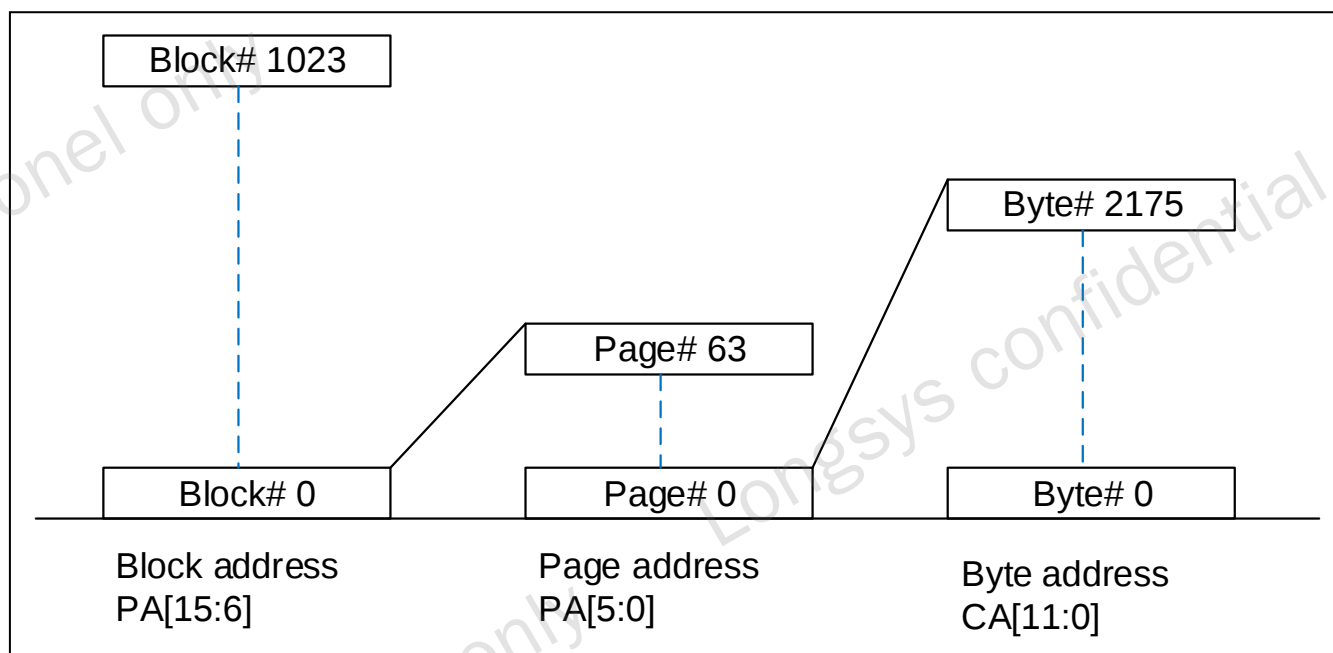
Figure 5 Address Mapping
