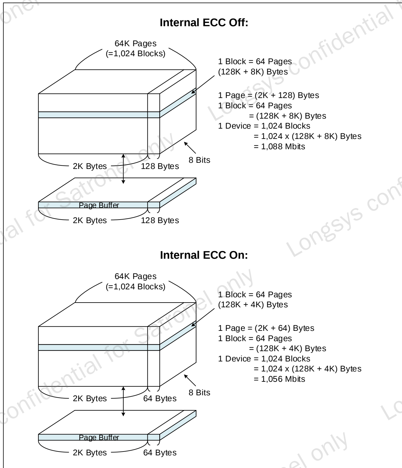
Figure 4 Array Organization
