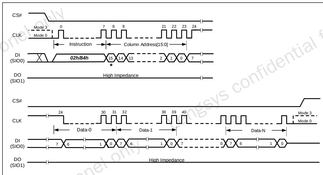
Figure 22 (Random) Program Data Load Sequence
