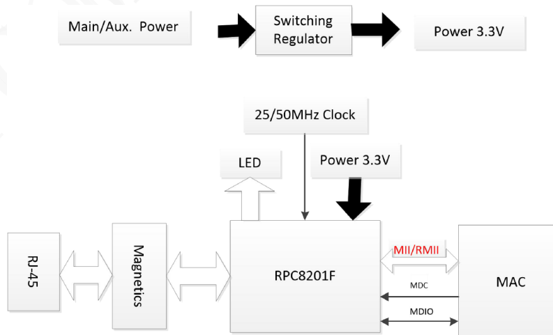
Figure 3-2 Block Diagram
