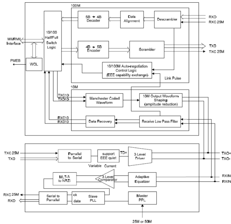
Figure 3-1 Block Diagram
