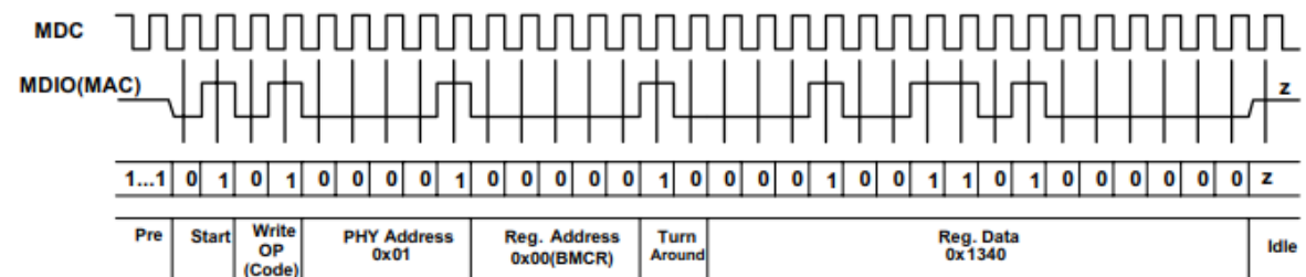
Figure7-2.Write Cycle
