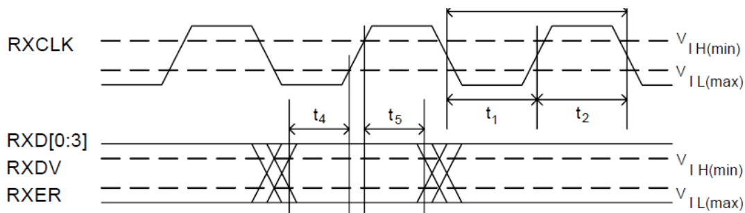
Figure 8-5. MII Reception Cycle Timing-1
