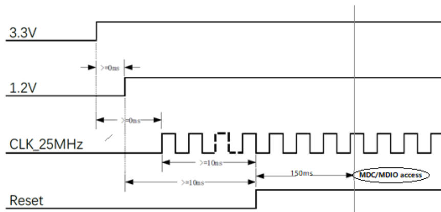
Figure 8-1. Power On and PHY Reset Sequence
