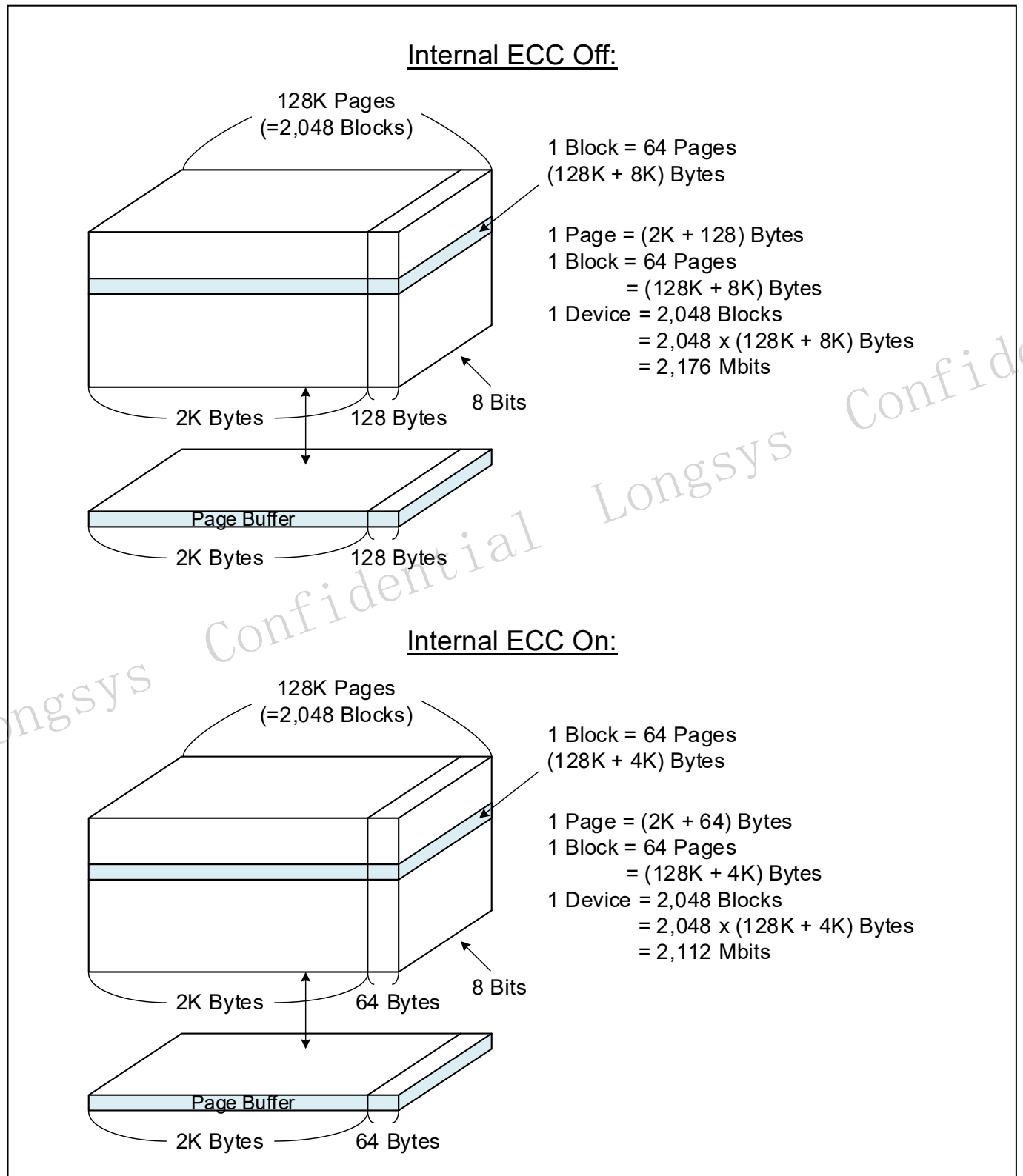
Figure 4 Array Organization
