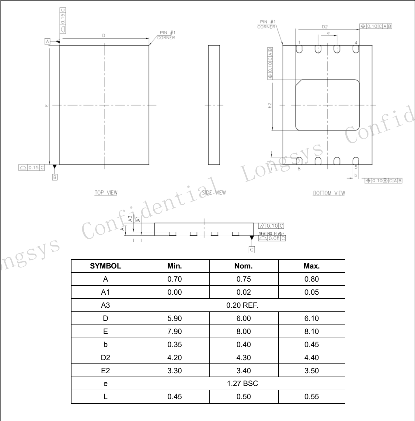
Figure 37 8-WSON (6x8mm) Package Information
