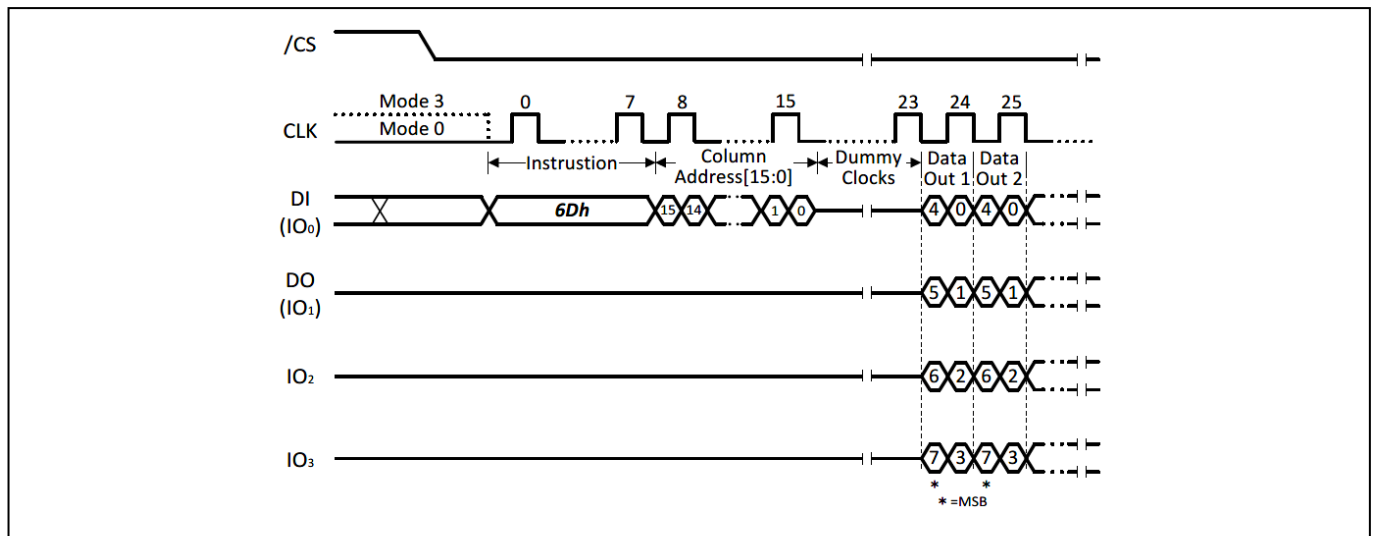
Figure 21 DTR Read Quad Output (6Dh) Sequence
