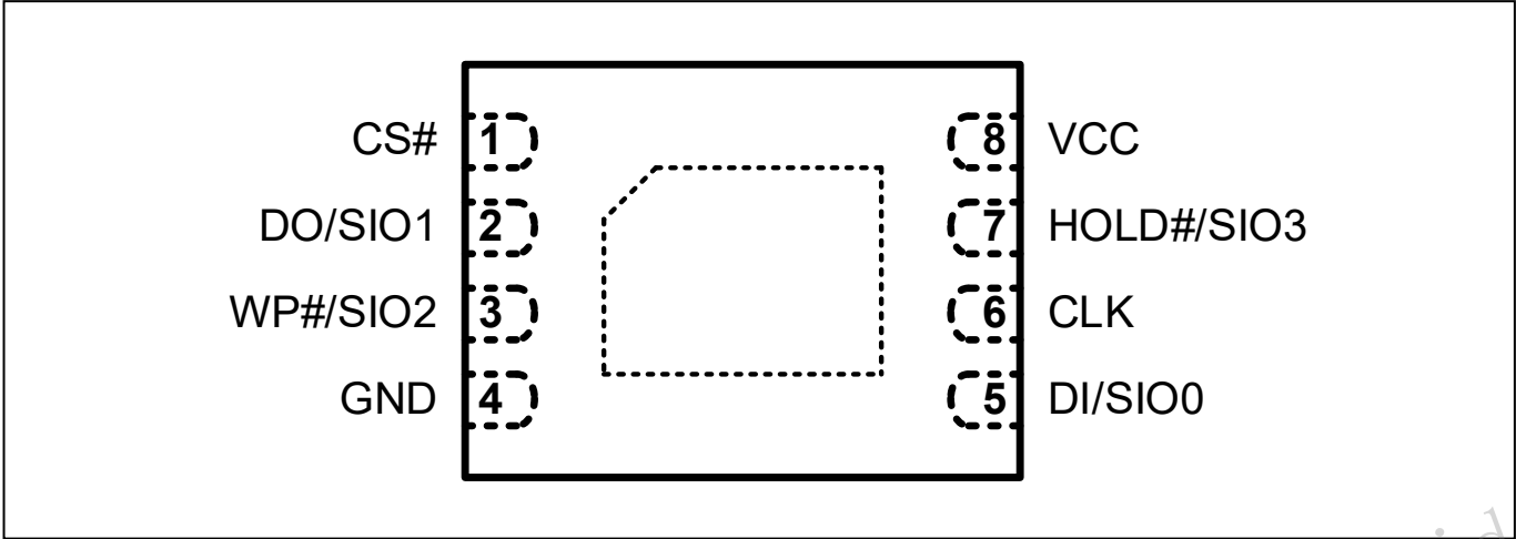
Figure 2 Pin Configuration 8-WSON (6x8mm)
