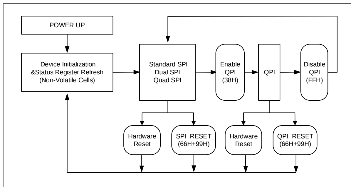
Figure 7-1 MH1128D Serial Flash Memory Operation Diagram
