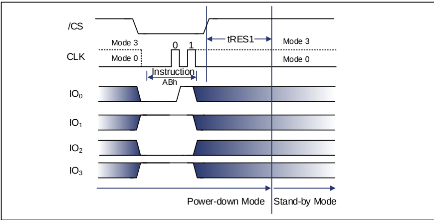
Figure 9-48 Release Power-down / Device ID Instruction (SPI Mode)
