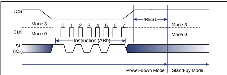
Figure 9-47 Release Power-down Instruction (QPI Mode)
