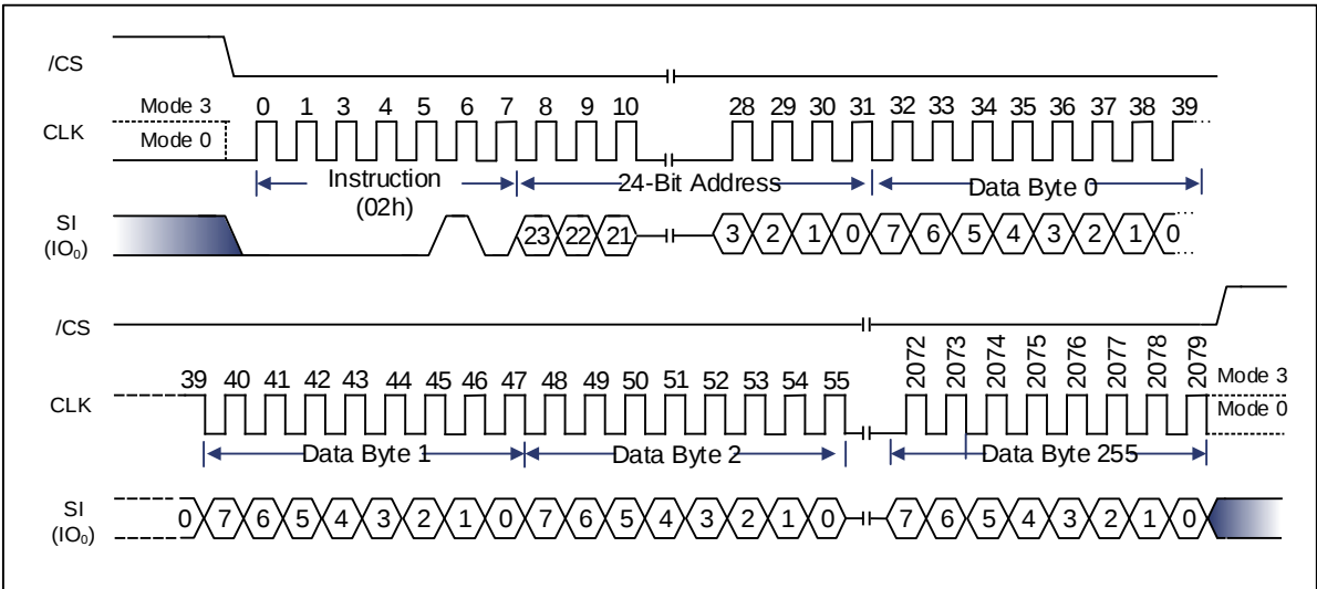
Figure 9-30 Page Program Instruction (SPI Mode)
