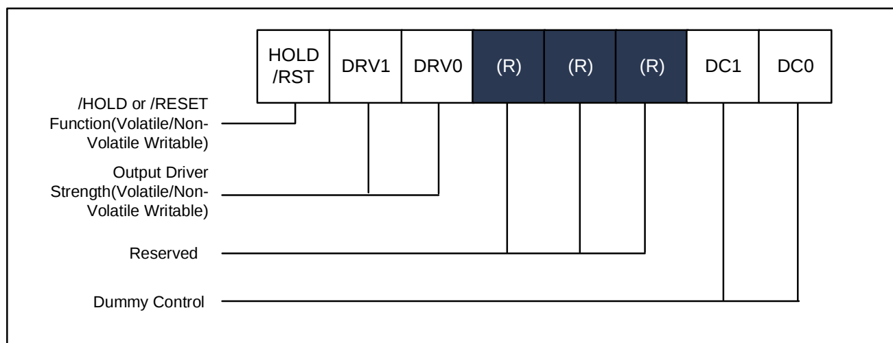
Figure 8-3 Status Register-3
