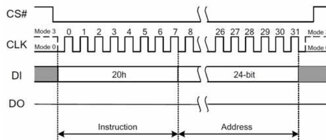
Figure 7.8a Sector Erase Instruction(SPI Mode)
