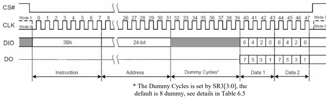
Figure 7.15 Fast Read Dual Output Instruction Sequence Diagram
