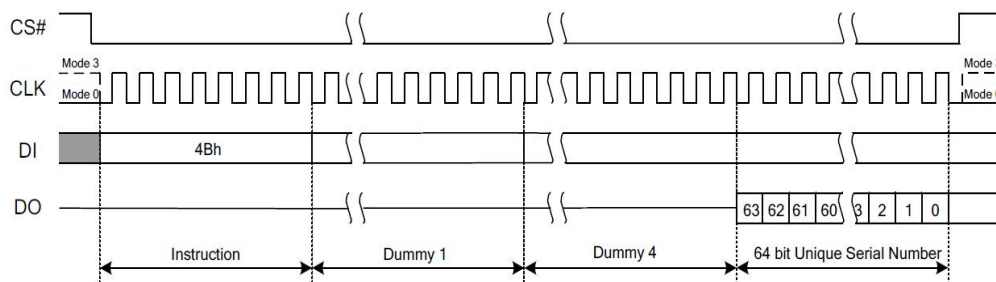
Figure 7.38 Read unique ID Number Instruction
