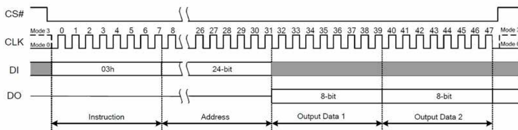
Figure 7.13 Read Data Instruction
