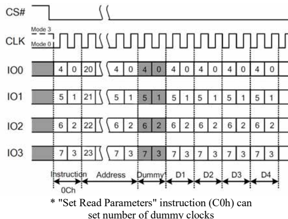
Figure 7.40 Burst Read with Wrap Instruction (QPI Mode only)
