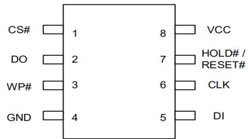
Figure 3.1 SOP8 (208mil)
