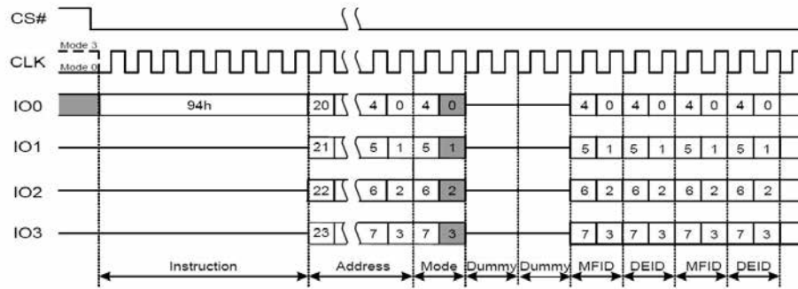
Figure 7.37 Read Manufacturer/Device ID Quad I/O Instruction
