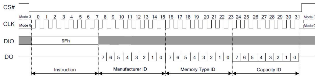
Figure 7.31a Read JEDEC ID(SPI Mode)
