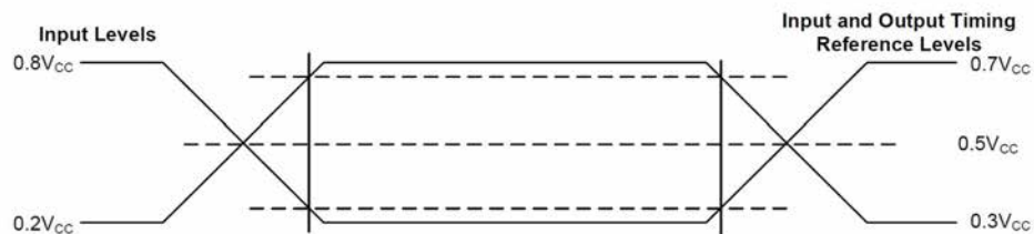
Figure 8.3 AC Measurement I/O Waveform
