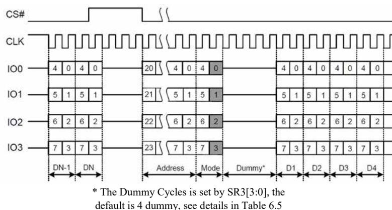
Figure 7.20 Fast Read Quad I/O Instruction(Previous command set M5-4 = 10)
