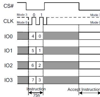
Figure 7.11b Erase / Program Suspend Instruction(QPI Mode)
