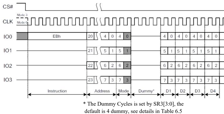
Figure 7.19a Fast Read Quad I/O Instruction(Initial command or previous M5-4 ≠10)
