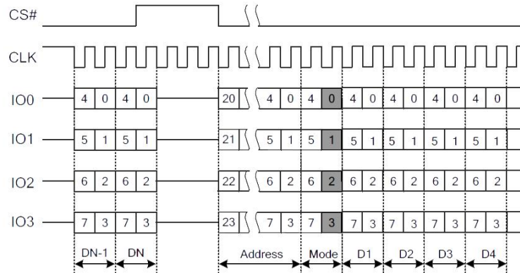
Figure 7.25 Set Burst with Wrap Instruction
