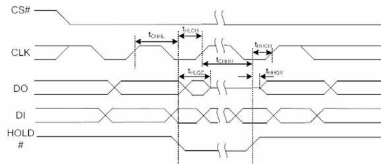
Figure 8.6 HoldTiming
