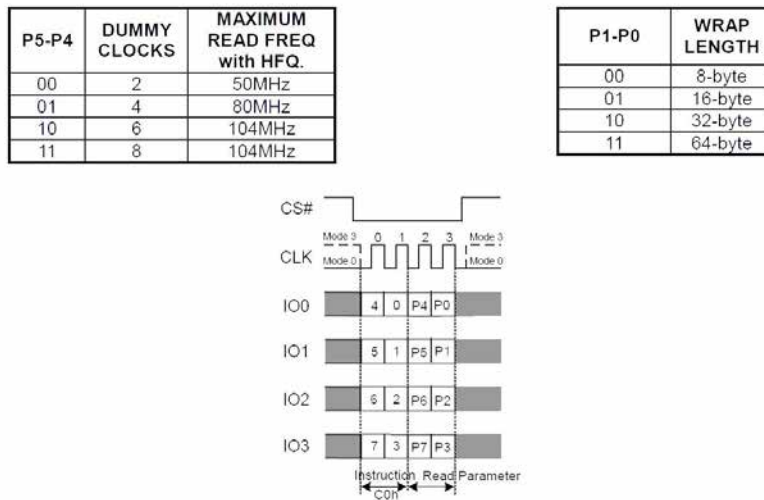
Figure 7.39 Set Read Parameters Instruction (QPI Mode only)
