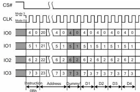
Figure 7.14b Fast Read Instruction (QPI Mode)
