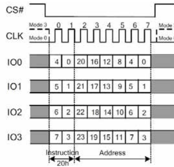
Figure 7.8b Sector Erase Instruction(QPI Mode)
