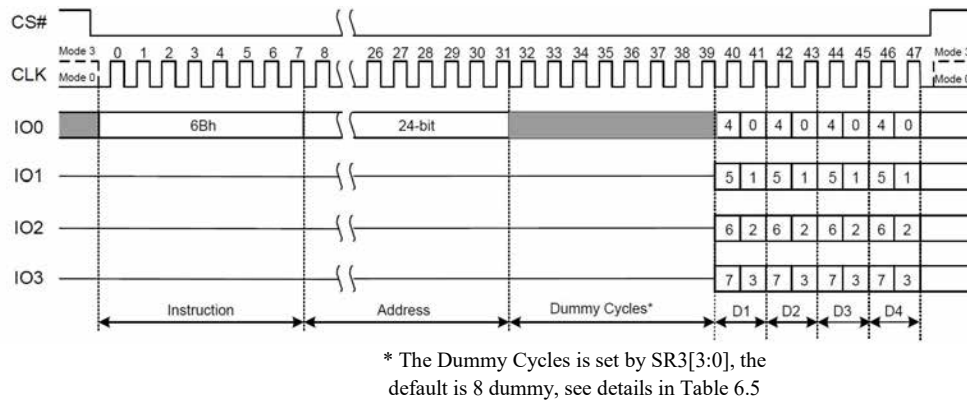
Figure 7.16 Fast Read Quad Output Instruction
