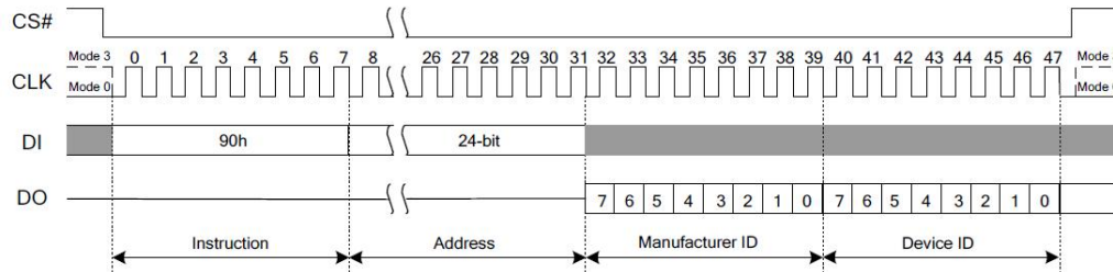
Figure 7.30a Read Manufacturer/Device ID(SPI Mode)
