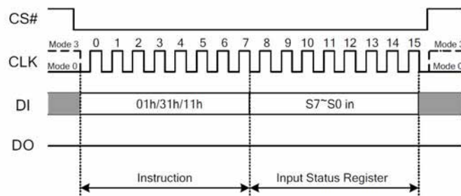
Figure 7.5a Write Status Register Instruction(SPI Mode)
