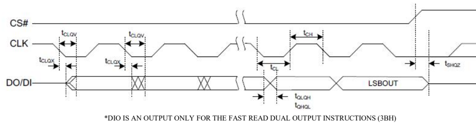
Figure 8.4 Serial Output Timing
