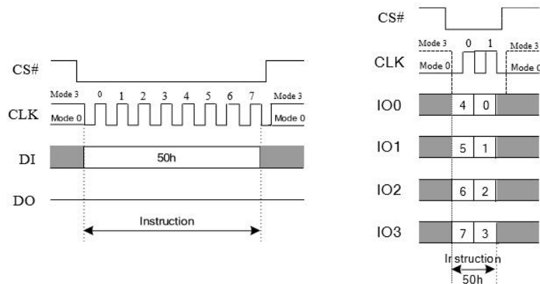
Figure 7.3 Write Enable for Volatile Status Register Instruction(SPI or QPI Mode)
