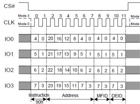
Figure 7.30b Read Manufacturer/Device ID(QPI Mode)
