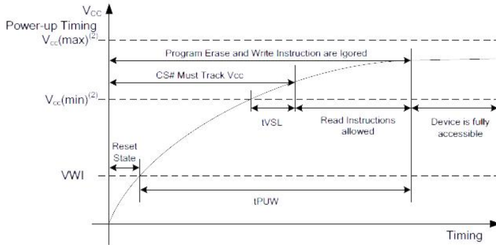
Figure 8.1 Power-up Timing
