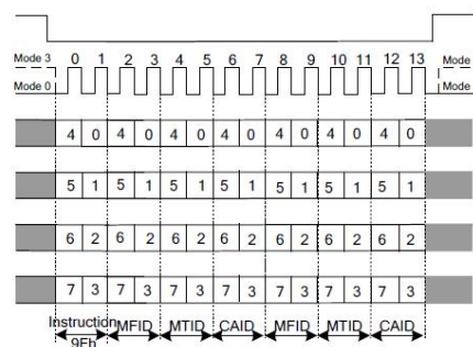
Figure 7.31b Read JEDEC ID(QPI Mode)
