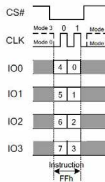
Figure 7.42 Exit QPI Instruction (QPI Mode only)
