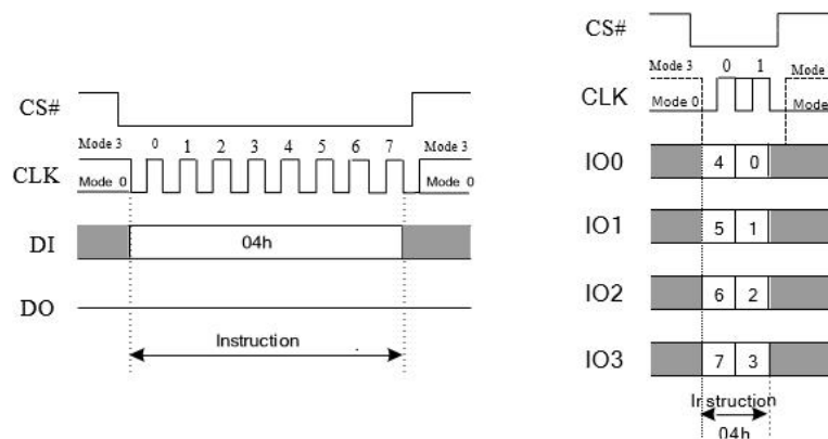
Figure 7.4 Write Disable Instruction(SPI or QPI Mode)
