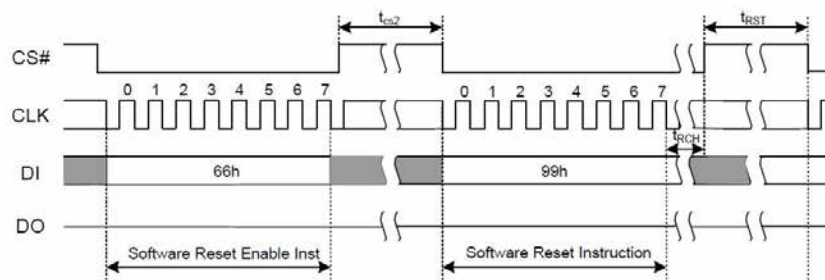
Figure 8.7 Software Reset Input Timing
