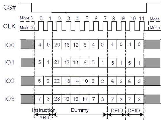
Figure 7.29b Release Power-down / Device ID(QPI Mode)
