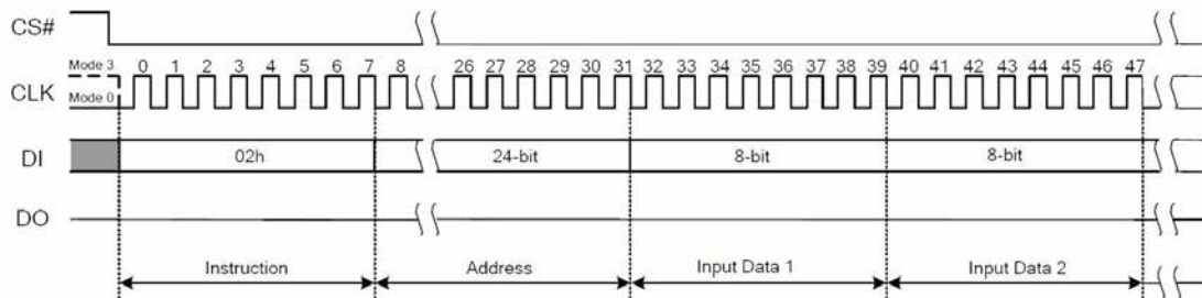
Figure 7.6a Page Program Instruction (SPI Mode)
