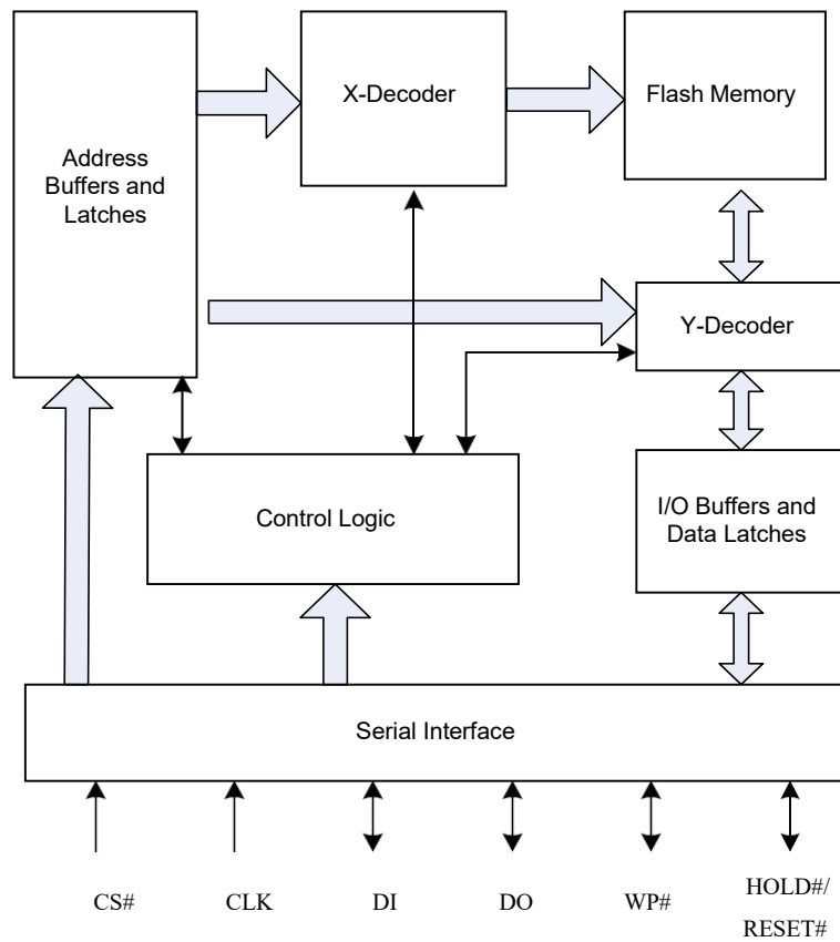
Figure 2.1 Block Diagram
