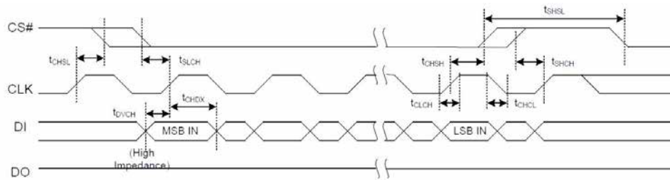
Figure 8.5 Input Timing
