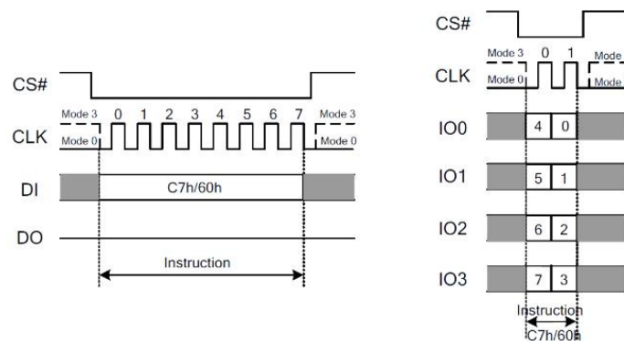
Figure 7.10 Chip Erase Instruction(SPI or QPI Mode)
