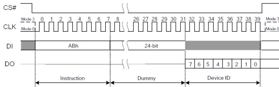
Figure 7.29a Release Power-down / Device ID(SPI Mode)
