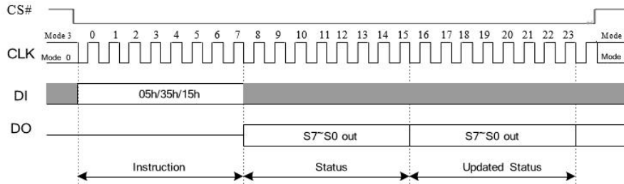
Figure 7.1a Read Status Register Instruction(SPI Mode)
