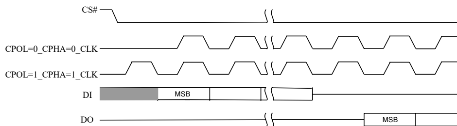
Figure 6.1 SPI Modes
