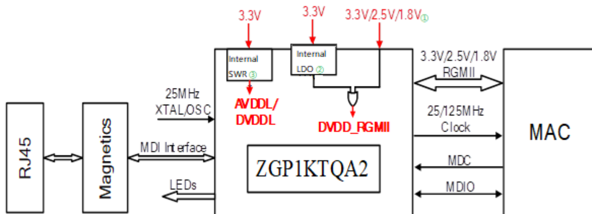
Figure 1. Application Diagram
